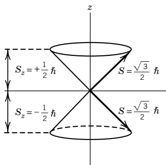
Figure 10.9 Possible orientations for the spin angular momentum \mathbf{S} of the electron in a magnetic field. The magnitude S of the spin angular momentum is [s(s + 1)]^{1/2}\hbar , where s is the spin quantum number. Thus, S = (\sqrt{3}/2)\hbar . The z component S_z of the spin angular momentum vector is m_s \hbar , where the spin quantum number m_s for the z is \pm 1/2 .
