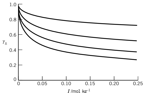
Figure 7.4 Mean ionic activity coefficients \gamma_{\pm} for electrolytes with z_+z_- = -1, -2, -3 , and -4 as a function of ionic strength I according to the extended Debye–Hückel equation. (See Computer Problem 7.E.)
