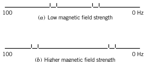
Figure 15.15 NMR spectrum of a molecule with two interacting hydrogen atoms. Note that the splitting is independent of the magnetic field strength.
