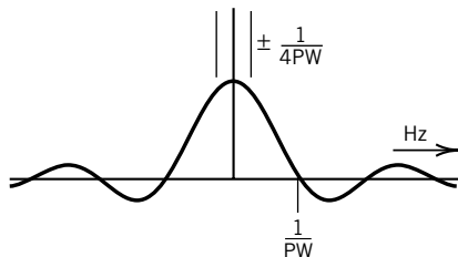
Figure 15.6 The effectiveness of a pulse of length PW versus frequency. The effectiveness is essentially constant in the range \pm 1/4PW . [From J. W. Akitt and B. E. Mann, NMR and Chemistry , Taylor and Francis Books Ltd. (Nelson Thornes), London, ©2000.]
