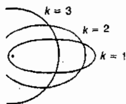
Fig. 1.5 Bohr-Sommerfeld orbits for n = 3 .
