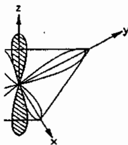
8 d^8 arrangement, d_{z^2} . (The d_{x^2-y^2} orbital is empty.)
