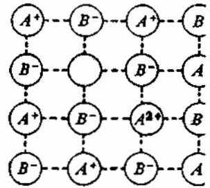
Figure 3.17 Metal deficiency caused by missing positive ion
