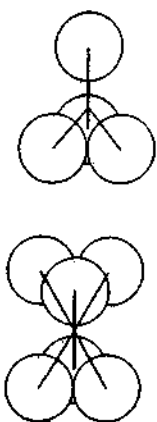
Tetrahedral and octahedral holes: (a) tetrahedral sites in a close-packed arrangement; (b) tetrahedral and octahedral sites.
