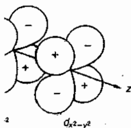
21 \delta bonding by d sideways overlap of two orbitals.
