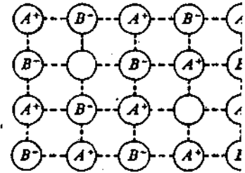
Figure 3.13 Schottky defect.
