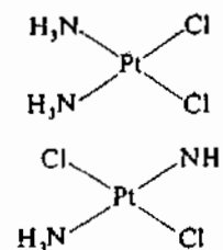
Figure 7.5 Isomerism in square planar complexes.
