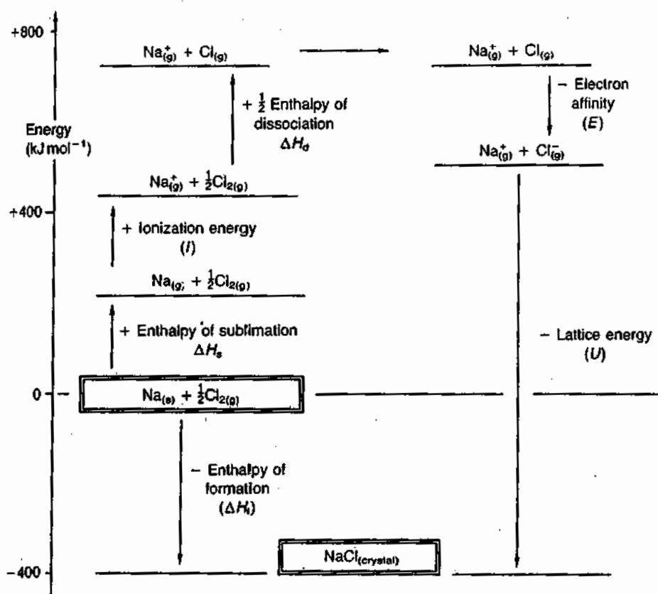
Figure 6.2 Born-Haber cycle for the formation of NaCl.
