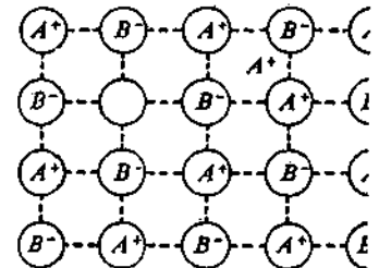
Figure 3.14 Frenkel defect.
