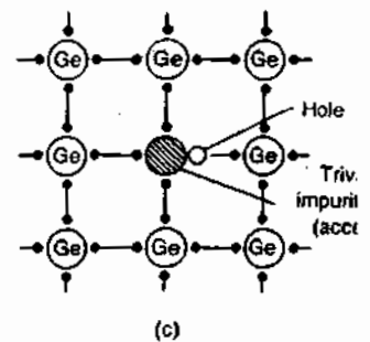
Figure 3.19 (a) Pure germanium. (b) n -type germanium. (c) p -type germanium.
