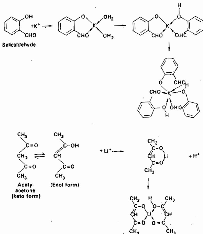
Figure 9.5 Salicylaldehyde and acetylacetone complexes.
