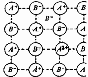
Figure 3.18 Metal deficiency caused by interstitial negative ions.
