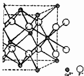
3.7 Fluorite ( \text{CaF}_2 ) structure. (Reproduced by permission of Wells, A.F., Inorganic Chemistry , Oxford University Press, 1984.)
