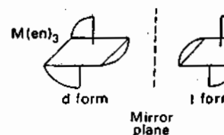
Figure 7.4 Optical isomerism octahedral complexes.
