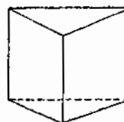
Trigonal prism
