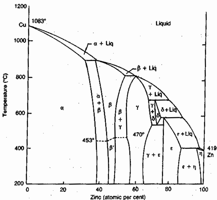
Figure 5.9 Phase diagram for Cu/Zn alloy systems. (Copyright Böhm and Klemm, Z. Anorg. Chem. , 243, 69, 1939.)
